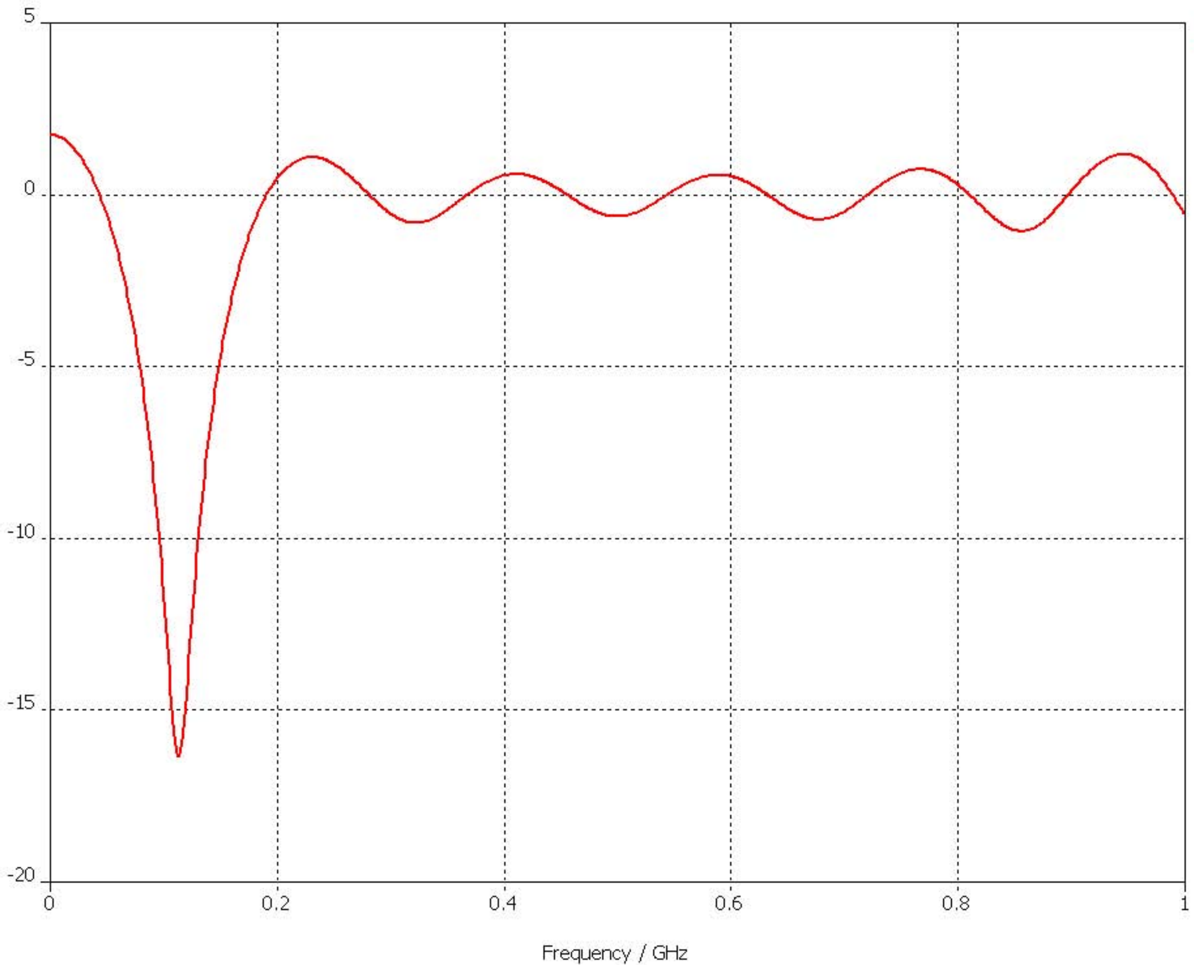
S-Parameter Magnitude in dB
