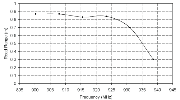
Figure 4: Read range measured over a frequency range
