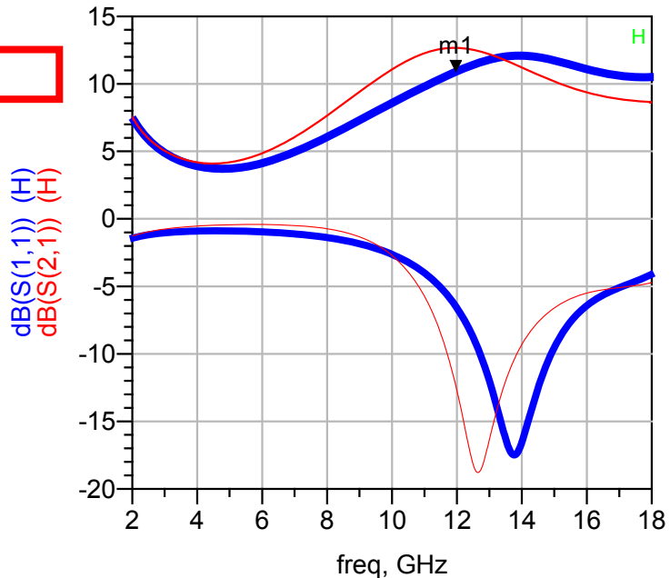
Forward Transmission, dB
