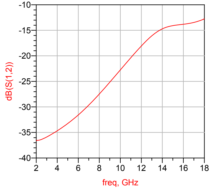
Reverse Transmission, dB
